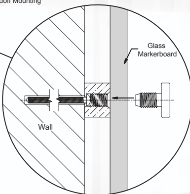
Standoff Mounting
